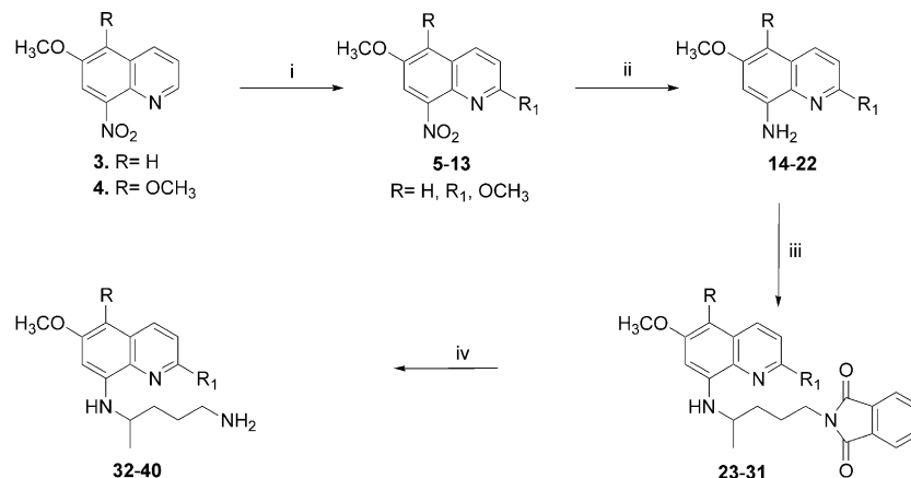
Scheme 1. Reagents and conditions: (i) \text{R}_1\text{CO}_2\text{H} , \text{AgNO}_3 , (\text{NH}_4)_2\text{S}_2\text{O}_8 , 10% \text{H}_2\text{SO}_4 , \text{CH}_3\text{CN} , 70^\circ\text{C} ; (ii) Raney Ni, EtOH, \text{H}_2 , 45 psi, 45 min; (iii) 2-(4-bromopentyl)-1,3-isoindolinedione, \text{Et}_3\text{N} , 120^\circ\text{C} , 24 h; (iv) \text{NH}_2\text{NH}_2 \cdot \text{H}_2\text{O} , EtOH, reflux, 8 h.
