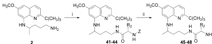
Scheme 2. Reagents and conditions: (i) Z-L- \text{R}_2 -OH, DCC, \text{CH}_2\text{Cl}_2 , rt; (ii) \text{H}_2 /Pd-C, 1 h, rt.
